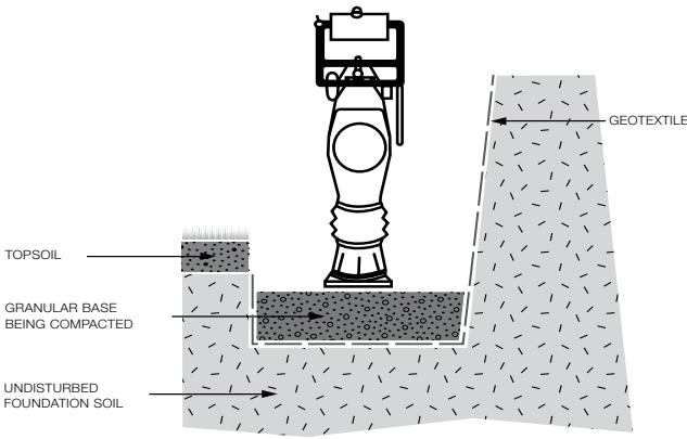
Figure 32. Base compaction
