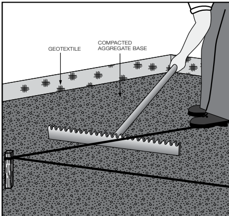
Figure 14. Use a grading rake for checking grades
