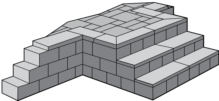
Figure 46. Protruding steps
